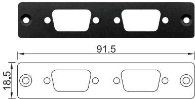
UB1603 Universal Bracket with 2x DB9 Cutout Dimension (WxD): 91.5 x 18.5 mm
