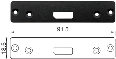
UB1606 Universal Bracket with DP Cutout Dimension (WxD): 91.5 x 18.5 mm
