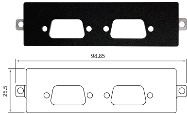
UB1403 Universal Bracket with 4x DB9 Cutout Dimension (WxD): 98.85 x 25.5 mm
