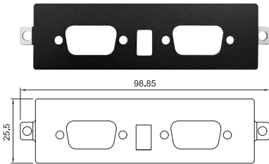
UB1438 Universal Bracket with 2x DB9 and 1x Switch Cutout for CMI-CAN Expansion Dimension (WxD): 98.85 x 25.5 mm
