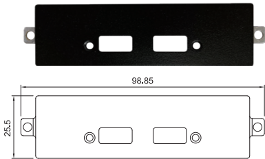
UB1414 Universal Bracket with 2x USB Cutout Dimension (WxD): 98.85 x 25.5 mm
