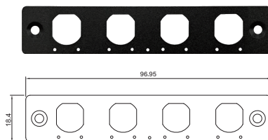
UB0930 Universal Bracket with 4x M12 X-Coded Cutout for DX Series Dimension (WxD) : 96.95 x 18.4 mm
