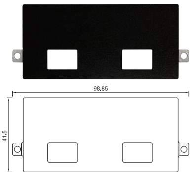
UB1828 Universal Bracket with 2x RJ45 Cutout Dimension (WxD): 98.85 x 41.5 mm
