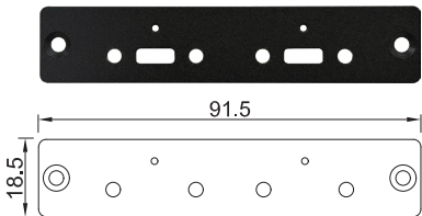
UB1633 Universal Bracket with 2x USB Type C Cutout for MEC-USB (M.2 interface) Expansion Dimension (WxD): 91.5 x 18.5 mm
