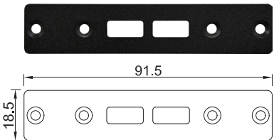
UB1634 Universal Bracket with 2x USB Type A Cutout for MEC-USB (M.2 interface) Expansion Dimension (WxD): 91.5 x 18.5 mm
