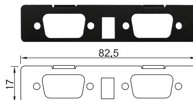
UB1538 Universal Bracket with 2x DB9 and 1x Switch Cutout for CMI-CAN Expansion Dimension (WxD): 82.5 x 17 mm
