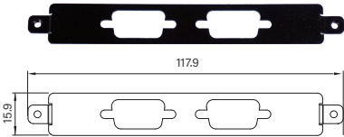
UB1203 Universal Bracket with 2x DB9 Cutout Dimension (WxD) : 117.9 x 15.9 mm
