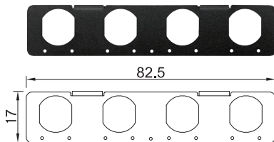
UB1510 Universal Bracket with 4x M12 Cutout Dimension (WxD): 82.5 x 17 mm
