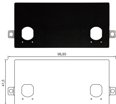
UB1837 Universal Bracket with 2x M12 X-coded Cutout Dimension (WxD): 98.85 x 41.5 mm
