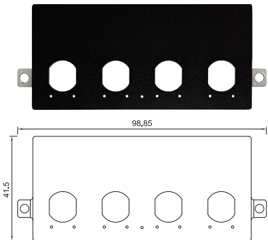
UB1810 Universal Bracket with 4x M12 Cutout Dimension (WxD): 98.85 x 41.5 mm
