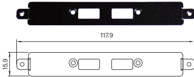
UB1214 Universal Bracket with 2x USB Cutout Dimension (WxD) : 117.9 x 15.9 mm
