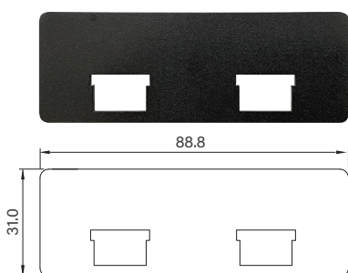
UB1028 Universal Bracket with 2x RJ45 Cutout Dimension (WxD) : 88.8 x 31 mm
