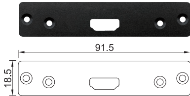
UB1608 Universal Bracket with HDMI® Cutout Dimension (WxD): 91.5 x 18.5 mm
