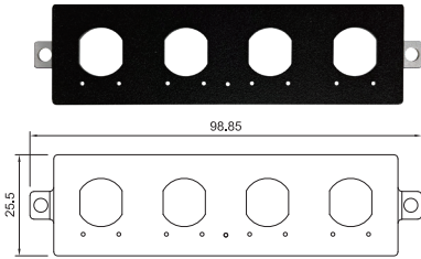
UB1410 Universal Bracket with 4x M12 Cutout Dimension (WxD): 98.85 x 25.5 mm
