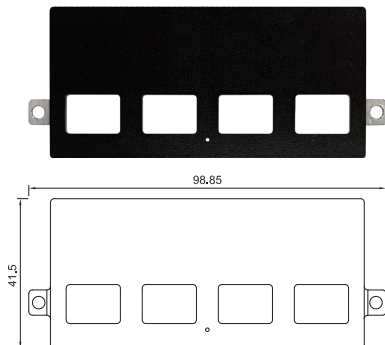
UB1812 Universal Bracket with 4x RJ45 Cutout Dimension (WxD): 98.85 x 41.5 mm
