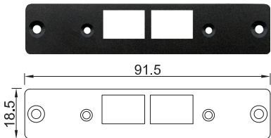
UB1611 Universal Bracket with 2x RJ45 Cutout Dimension (WxD): 91.5 x 18.5 mm
