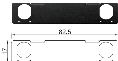
UB1537 Universal Bracket with 2x M12 X-coded Cutout Dimension (WxD): 82.5 x 17 mm
