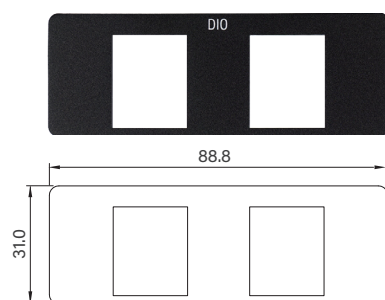
UB1018 Universal Bracket with DIO Cutout Dimension (WxD) : 88.8 x 31 mm
