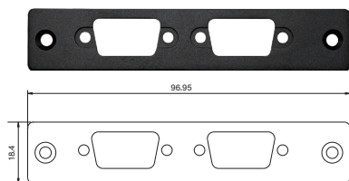
UB0903 Universal Bracket with 2x DB9 Cutout Dimension (WxD) : 96.95 x 18.4 mm
