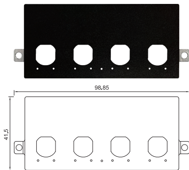
UB1830 Universal Bracket with 4x M12 X-Coded Cutout Dimension (WxD): 98.85 x 41.5 mm
