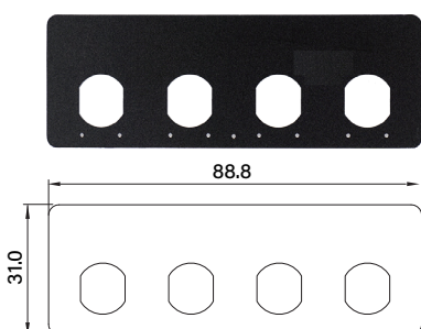
UB1010 Universal Bracket with 4x M12 Cutout Dimension (WxD) : 88.8 x 31 mm
