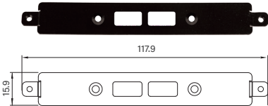
UB1234 Universal Bracket with 2x USB Type A Cutout for MEC-USB (M.2 interface) Expansion Dimension(WxD): 117.9 x 15.9 mm
