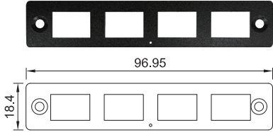
UB1712 Universal Bracket with 4x RJ45 Cutout Dimension (WxD): 96.95 x 18.4 mm
