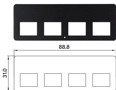
UB1012 Universal Bracket with 4x RJ45 Cutout Dimension (WxD) : 88.8 x 31 mm
