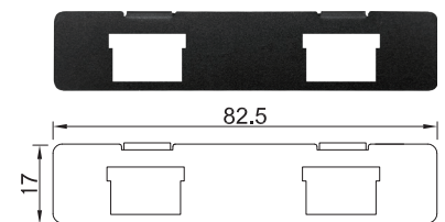
UB1528 Universal Bracket with 2x RJ45 Cutout Dimension (WxD): 82.5 x 17 mm
