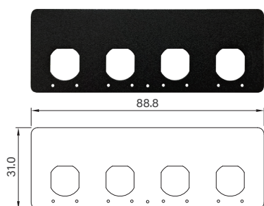
UB1030 Universal Bracket with 4x M12 X-Coded Cutout Dimension (WxD) : 88.8 x 31 mm
