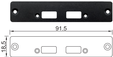
UB1614 Universal Bracket with 2x USB Cutout Dimension (WxD): 91.5 x 18.5 mm
