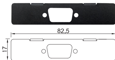
UB1516 Universal Bracket with VGA Cutout Dimension (WxD): 82.5 x 17 mm
