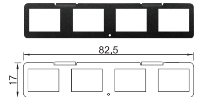
UB1512 Universal Bracket with 4x RJ45 Cutout Dimension (WxD): 82.5 x 17 mm
