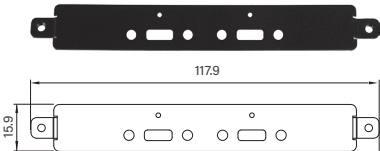
UB1233 Universal Bracket with 2x USB Type C Cutout for MEC-USB Expansion Dimension(WxD): 117.9 x 15.9 mm
