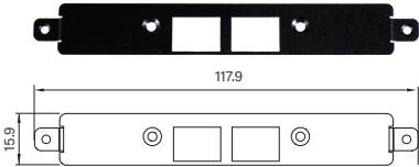
UB1211 Universal Bracket with 2x RJ45 Cutout Dimension (WxD) : 117.9 x 15.9 mm
