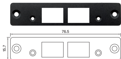
UB1911 Universal Bracket with 2x RJ45 Cutout for MEC-LAN Expansion (DC Series Front Bezel) Dimension (WxD): 76.5 x 15.7 mm
