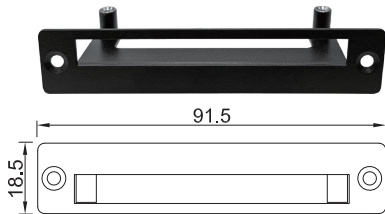
UB1618 Universal Bracket with DIO Cutout Dimension (WxD): 91.5 x 18.5 mm
