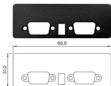
UB1038 Universal Bracket with 2x DB9 and 1x Switch Cutout for CMI-CAN Expansion Dimension (WxD) : 88.8 x 31 mm
