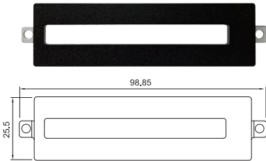
UB1418 Universal Bracket with DIO Cutout Dimension (WxD): 98.85 x 25.5 mm
