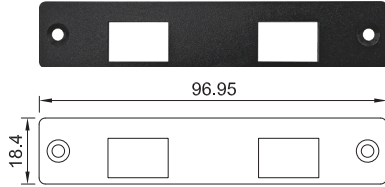
UB1728 Universal Bracket with 2x RJ45 Cutout for CMI-10GLAN Expansion Dimension (WxD): 96.95 x 18.4 mm
