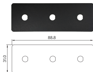
UB1032 Universal Bracket with 3x Antenna Cutout Dimension (WxD) : 88.8 x 31 mm
