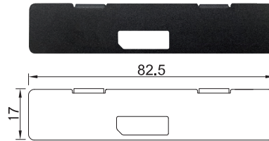
UB1506 Universal Bracket with DisplayPort Cutout Dimension (WxD): 82.5 x 17 mm
