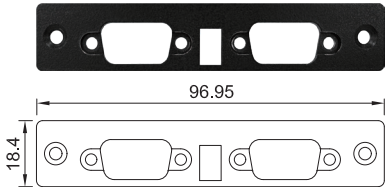
UB1738 Universal Bracket with 2x DB9 and 1x Switch Cutout for CMI-CAN Expansion Dimension (WxD): 96.95 x 18.4 mm
