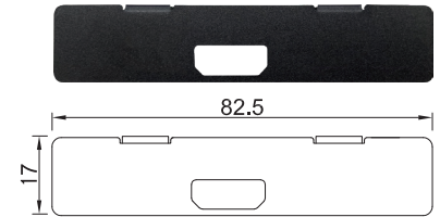
UB1508 Universal Bracket with HDMI® Cutout Dimension (WxD): 82.5 x 17 mm
