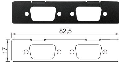
UB1503 Universal Bracket with 2x DB9 Cutout Dimension (WxD): 82.5 x 17 mm
