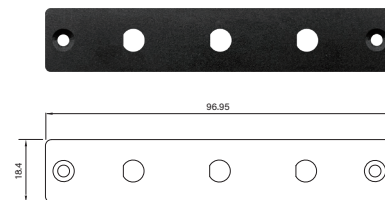
UB0932 Universal Bracket with 3x Antenna Cutout Dimension (WxD) : 96.95 x 18.4 mm
