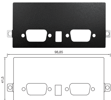
UB1838 Universal Bracket with 2x DB9 and 1x Switch Cutout for CMI-CAN Expansion Dimension (WxD): 98.85 x 41.5 mm
