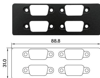
UB1004 Universal Bracket with 4x DB9 Cutout Dimension (WxD) : 88.8 x 31 mm
