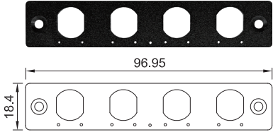
UB1710 Universal Bracket with 4x M12 A-Coded Cutout Dimension (WxD): 96.95 x 18.4 mm
