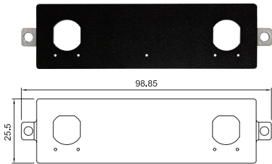
UB1437 Universal Bracket with 2x M12 X-coded Cutout Dimension (WxD): 98.85 x 25.5 mm
