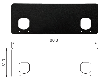
UB1037 Universal Bracket with 2x M12 X-coded Cutout Dimension (WxD) : 88.8 x 31 mm
