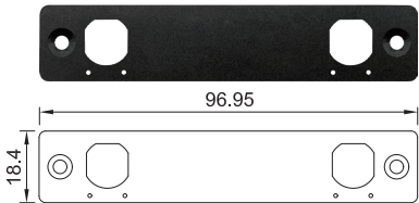
UB1737 Universal Bracket with 2x M12 X-coded Cutout Dimension (WxD): 96.95 x 18.4 mm
